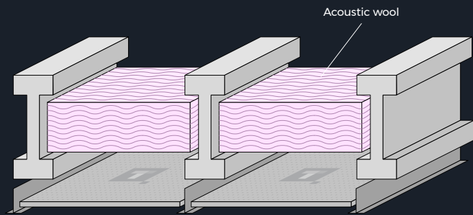
Scenario 1: Installation of T|Karra tiles with a minimum spacing of 6” between the joists and suspended ceiling.
